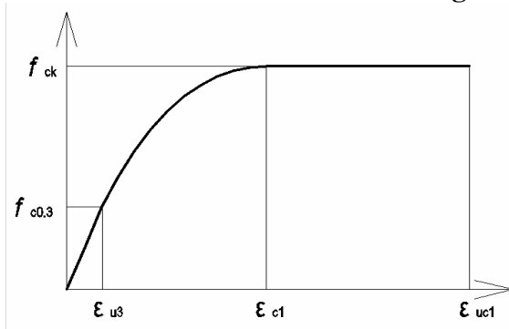
Fig. 6. Material properties
