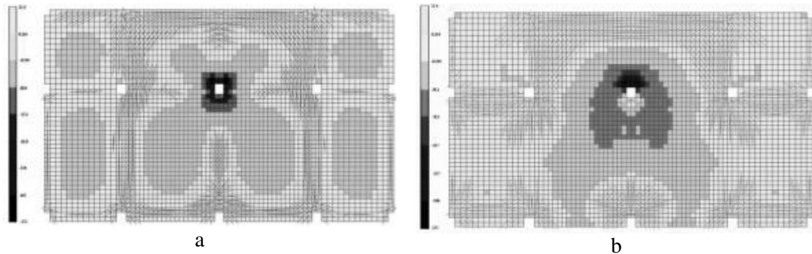
Fig. 19. Crack distribution in slabs adjacent to the damaged cells: a – Slab reinforced with ribs; b – Flat slab
