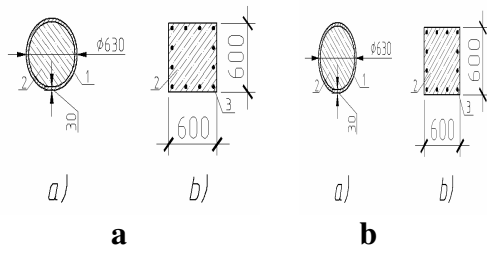
Fig. 10. Cross section: a – CFST; b – RRC; 1 – Steel tube; 2 – Concrete core 3 – Rebar
