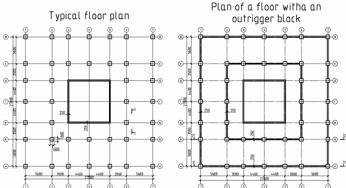
Fig. 3. Typical floor plan
