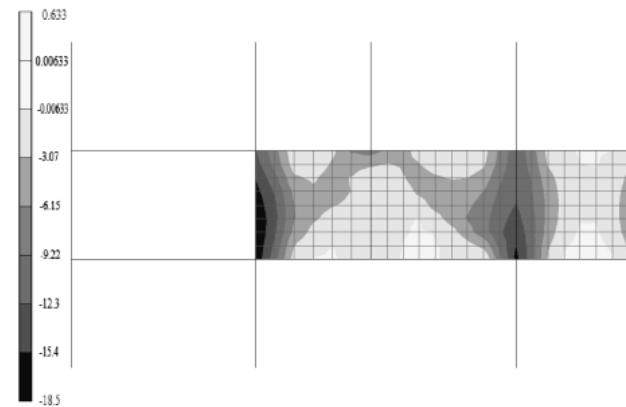
Fig. 15. Stress distribution in OB
