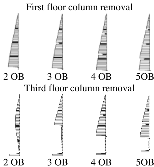
Fig. 14. Influence of amount of outrigger blocks (OB) on axial force distribution in columns
