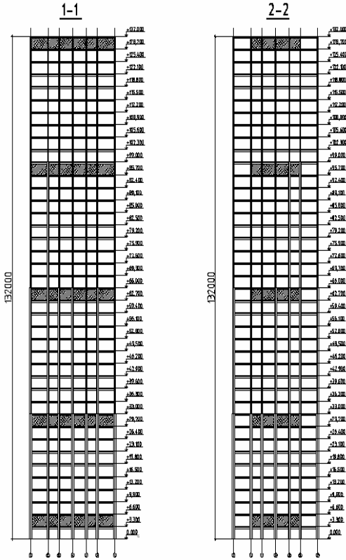
Fig. 4. Cross section
