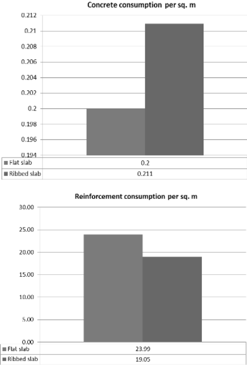
Fig. 21. Consumption of concrete m 3 /m 2 and reinforcement kg/m 2
