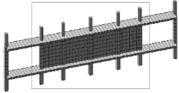
Fig. 7. Part of finite element model
