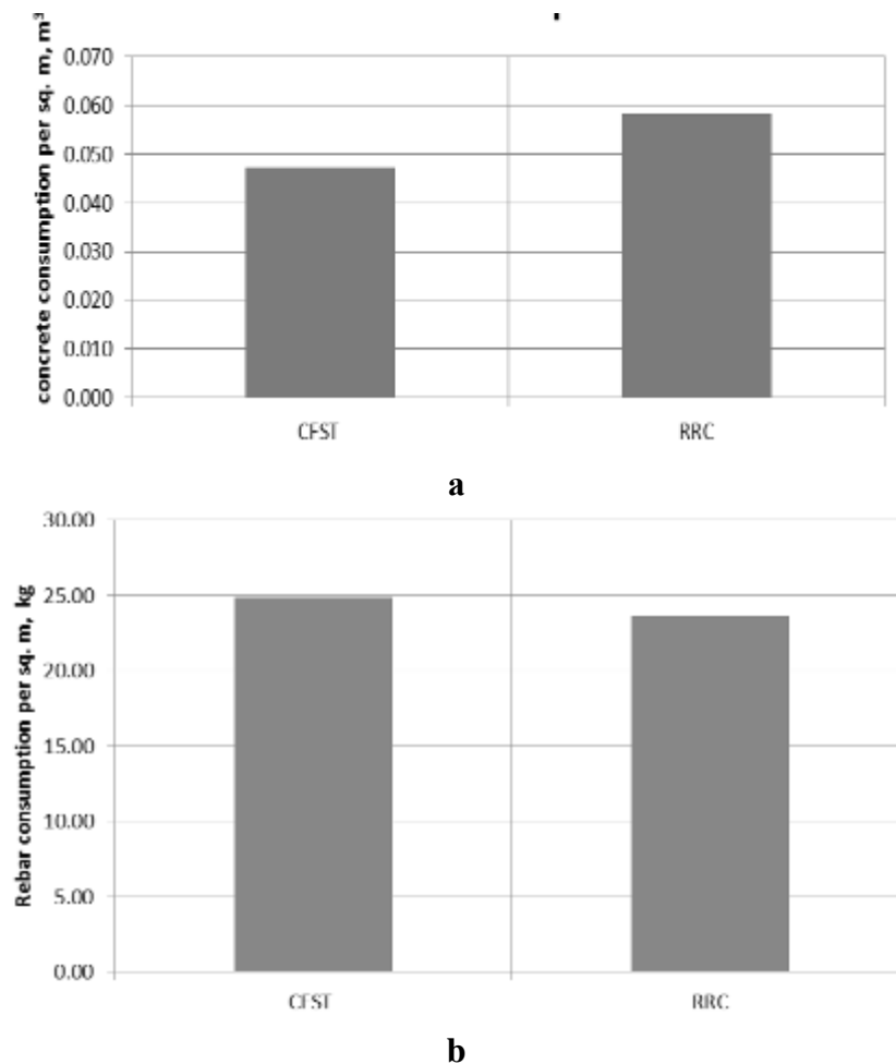
Fig. 22. Material consumption: a – Concrete consumption; b – Reinforcement consumption
