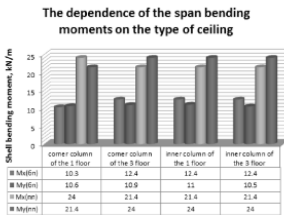
Fig. 18. Dependency of bending moments on the construction of the slab
