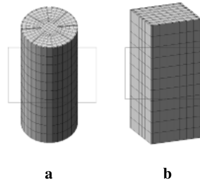
Fig. 13. Finite element model: a – CFST; b – RRC
