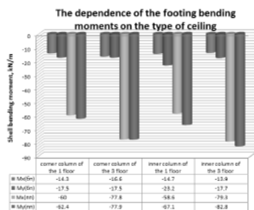
Fig. 18. Dependency of bending moments on the construction of the slab
