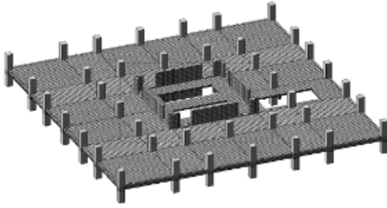
Fig. 8. Part of finite element model
